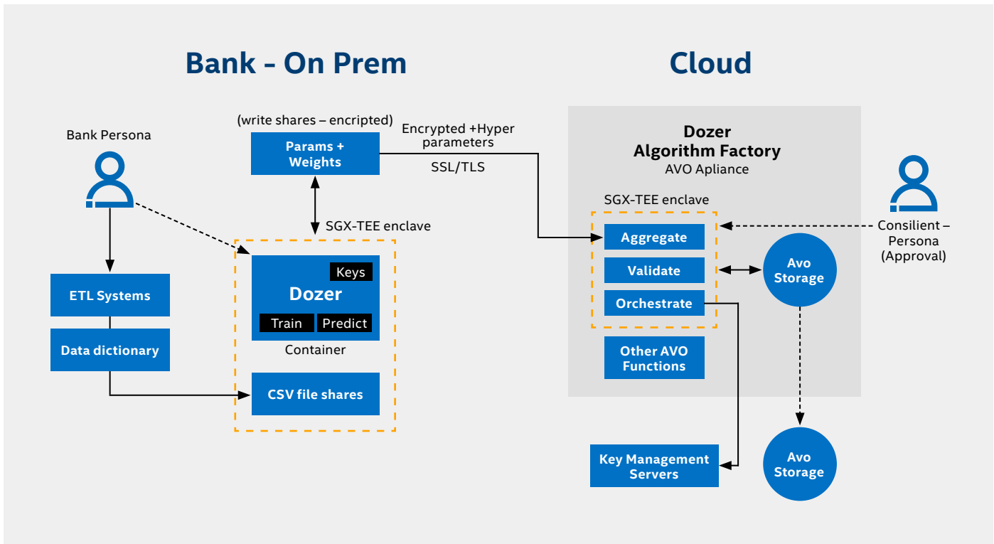
Figure 3. Secure Privacy-Preserving Federated Learning AML Solution Architecture
