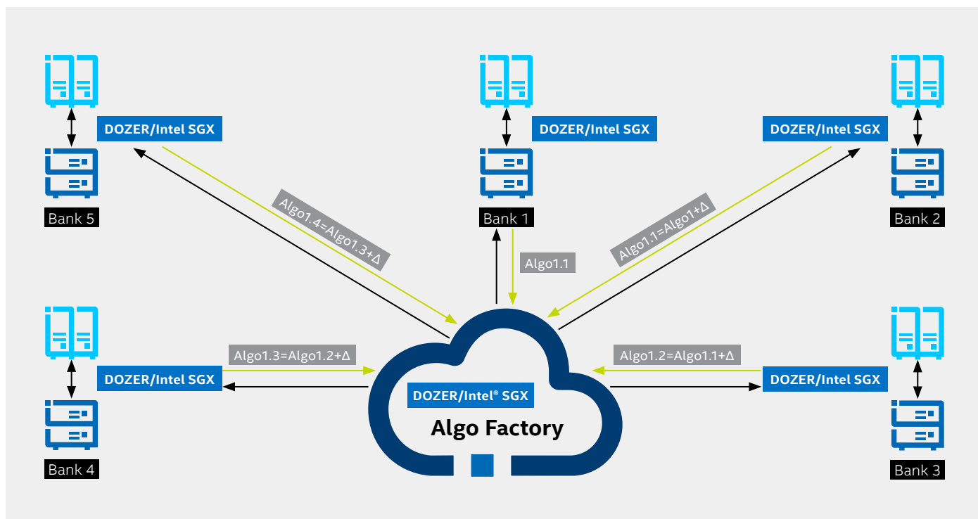
Figure 1. Consilient's Federated Learning Framework
