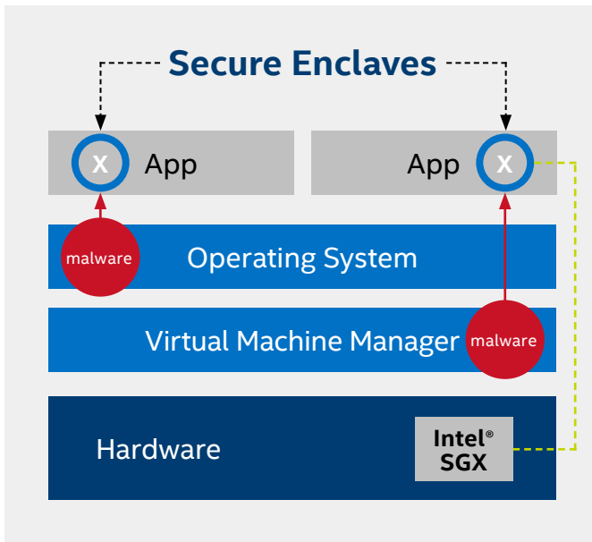
Figure 2. Intel® SGX Stack
